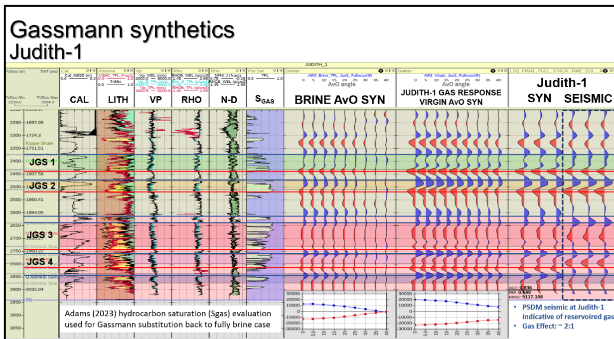
Figure 6: Judith-1 Gassman Synthetics showing brine saturation case and seismic response to gas saturation in Judith reservoirs. Gassmann synthetics and PDSM seismic indicative of gas on seismic at Judith-1.
